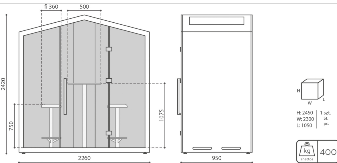
THS 2 SG1 / THSW 2 SG1
