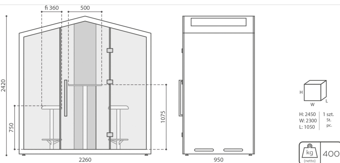
THS 2 SG2 / THSW 2 SG2
